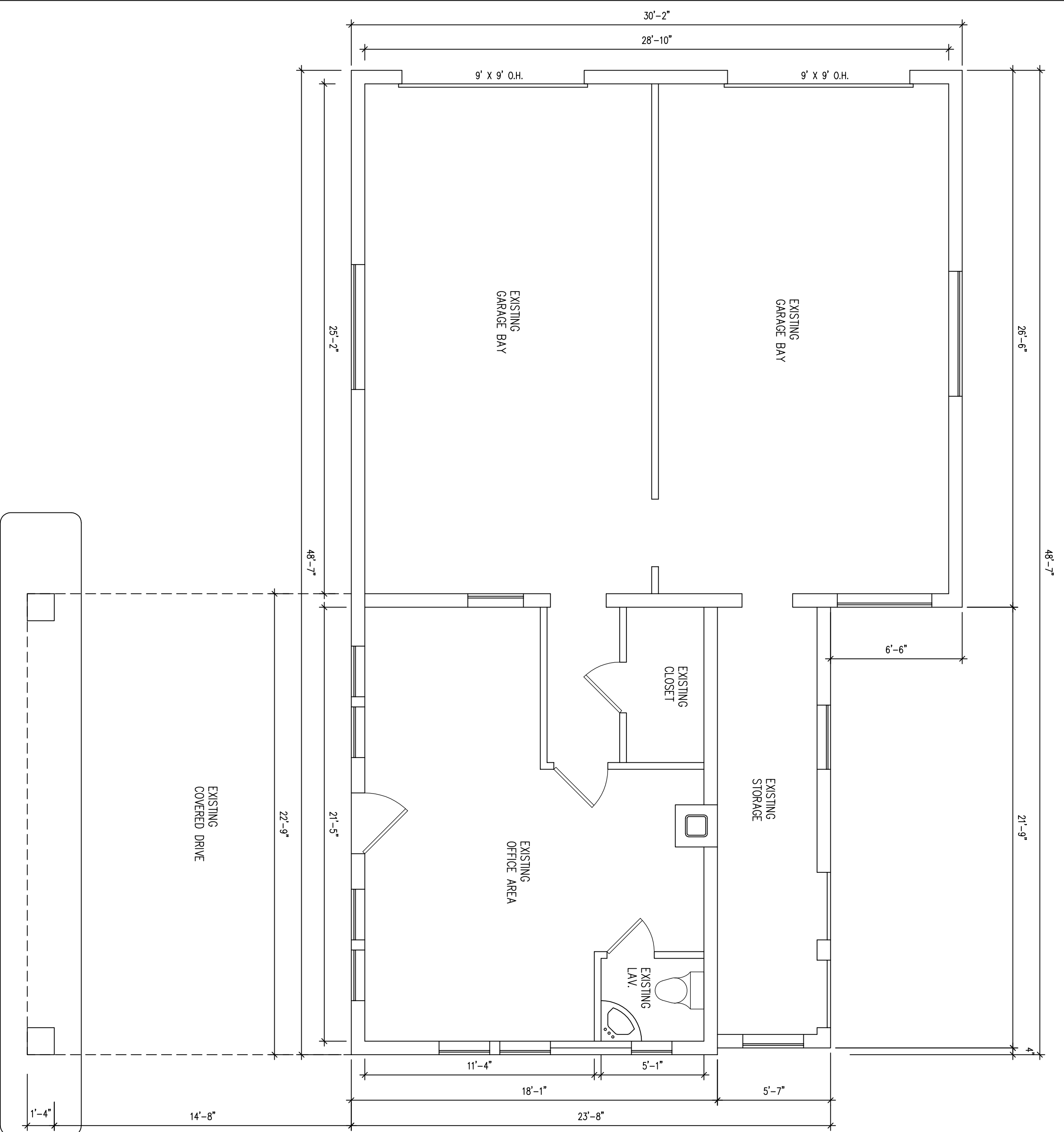
EXISTING FLOOR PLAN EXISTING FIRST FLOOR AREA = 1318 SQ. FT. SCALE: 1/4"=1'-0"
